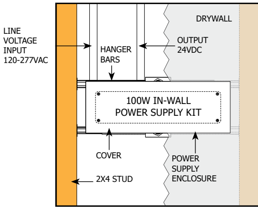
PSB-100W-ELV-24VDC-IW
