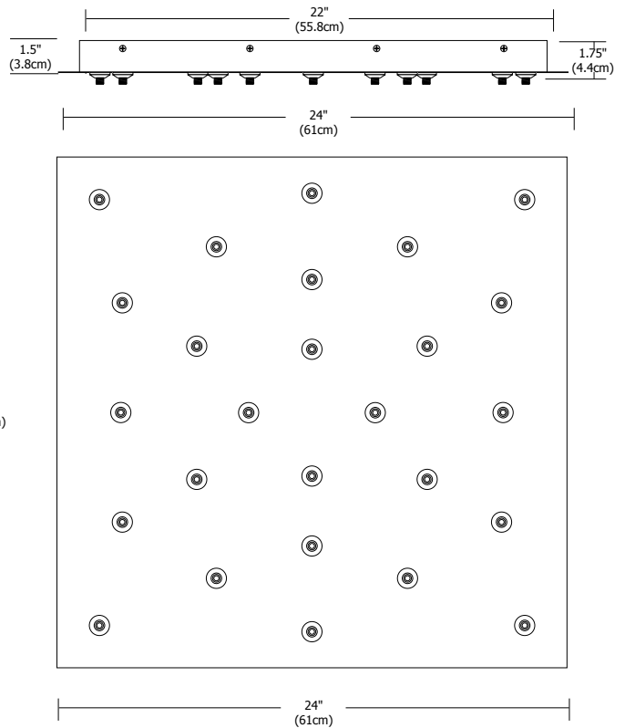
26-Port Canopy
