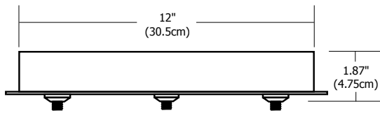
3 and 4 Port Round Canopy
