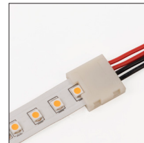
Snap the cover to secure in place
