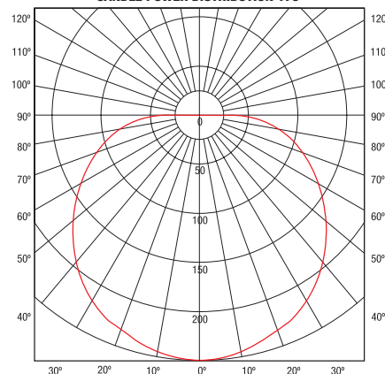
CANDLE POWER DISTRIBUTION 176°
