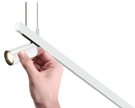
Teeny Track Head 702 lumens @3000K 2 5/8" Long x 1 5/16" Dia
