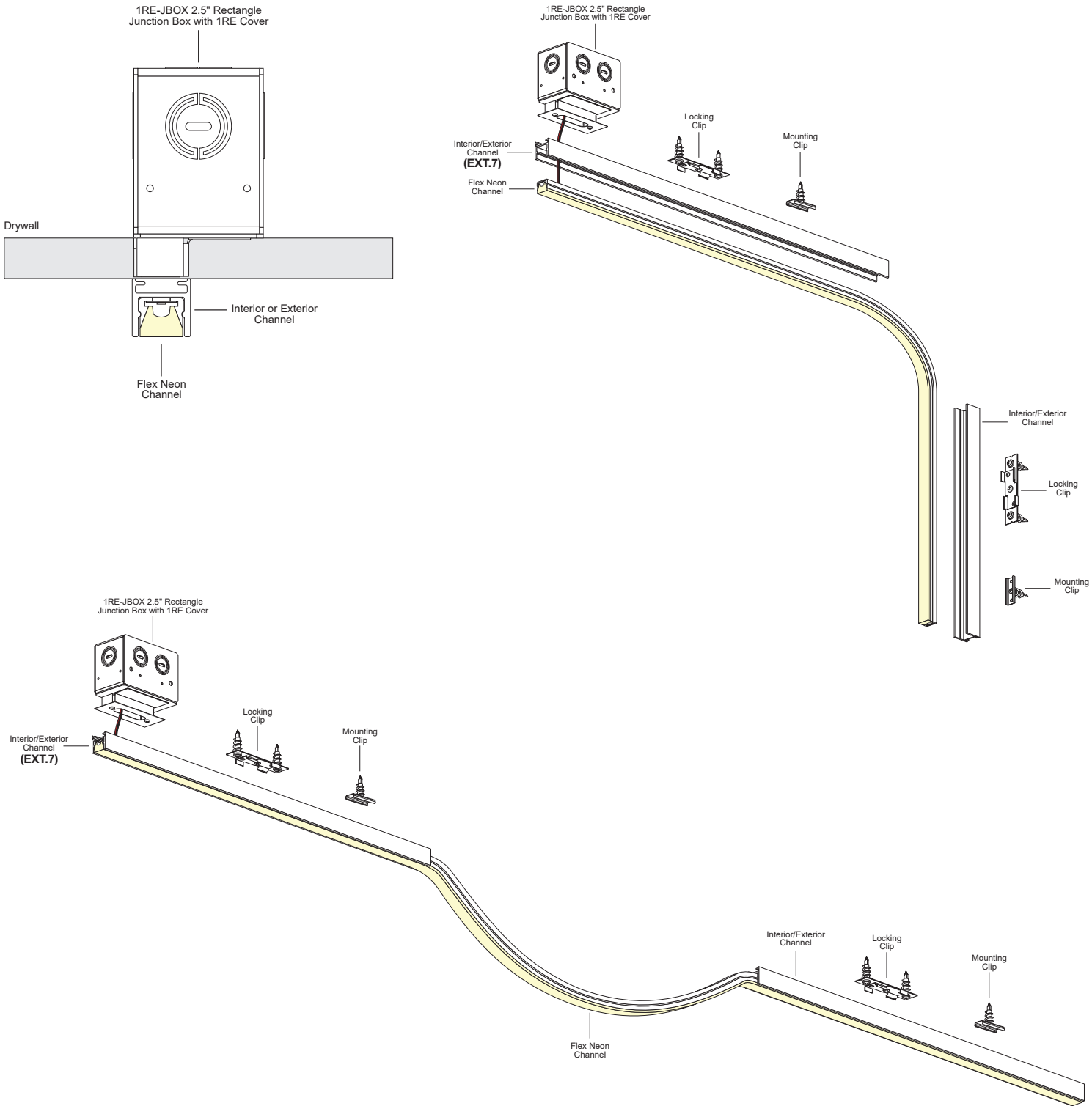
Drawings: Exploded View for Flexible Aluminum Channel with 1RE J-box
