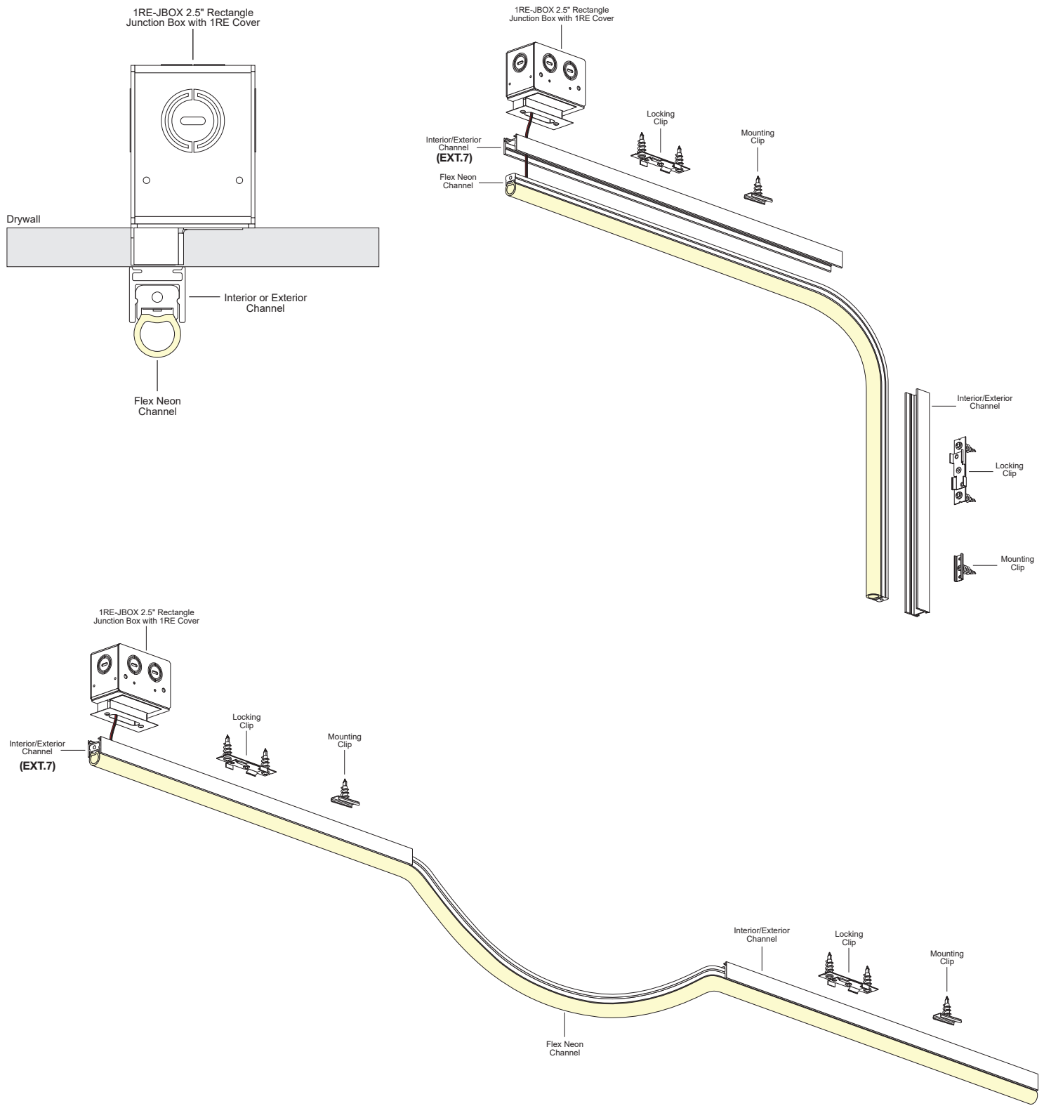
Drawings: Exploded View for Flexible Aluminum Channel with 1RE J-box
