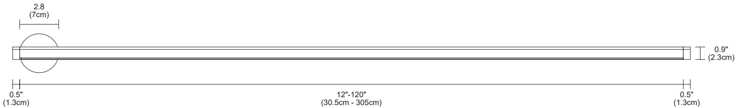
CIRRUS SUSPENSION WALL WASH WITH GLARE SHIELD AND WHITE LOUVER
