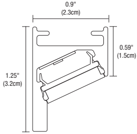
CIRRUS SUSPENSION WALL WASH WITH GLARE SHIELD AND LOUVER
