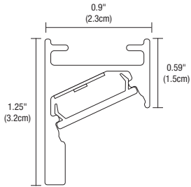
CIRRUS SUSPENSION WALL WASH WITH GLARE SHIELD
