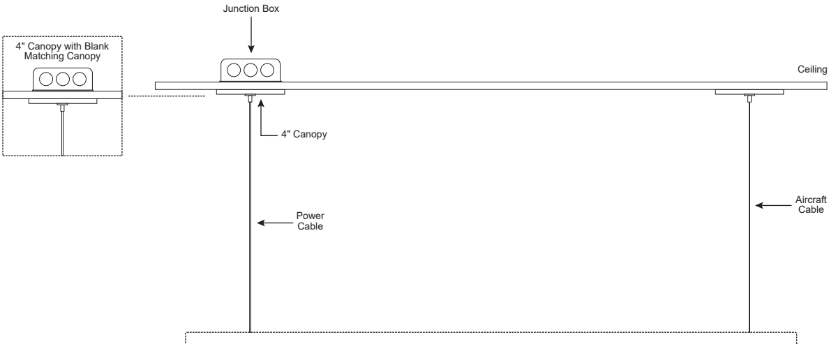
General 4S2 & 4R2 for Linear Suspension
