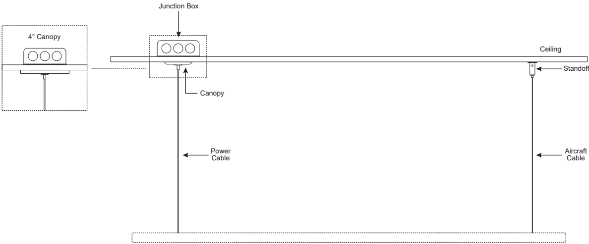
General End Feed for Linear Suspension
