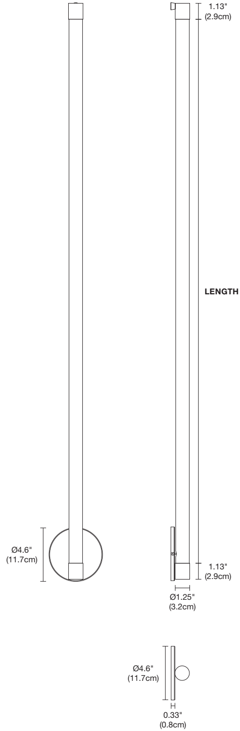
E4R - End Power Feed 4" Round Canopy
