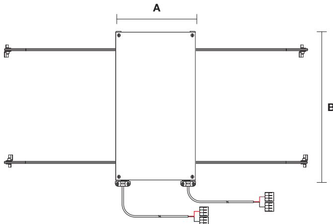
PSB-96W-010-24VDC-WDPS-TB (T-BAR GRID CEILING)
