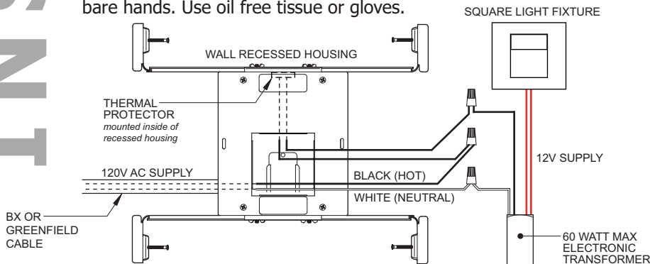
SQUARE LIGHT FIXTURE - image shown with faceplate removed for relamping.
